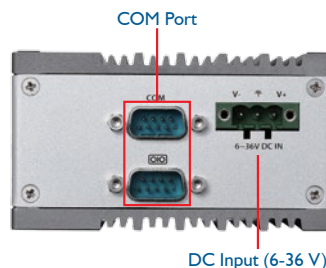
■ Right side view of MXE-200/200i
